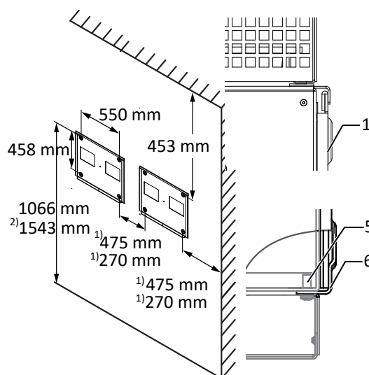
Abb. 12: Wandmontage
