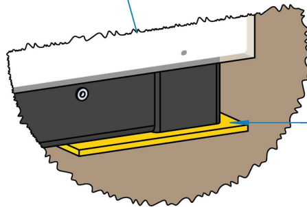
DETAIL C (1 : 8)
