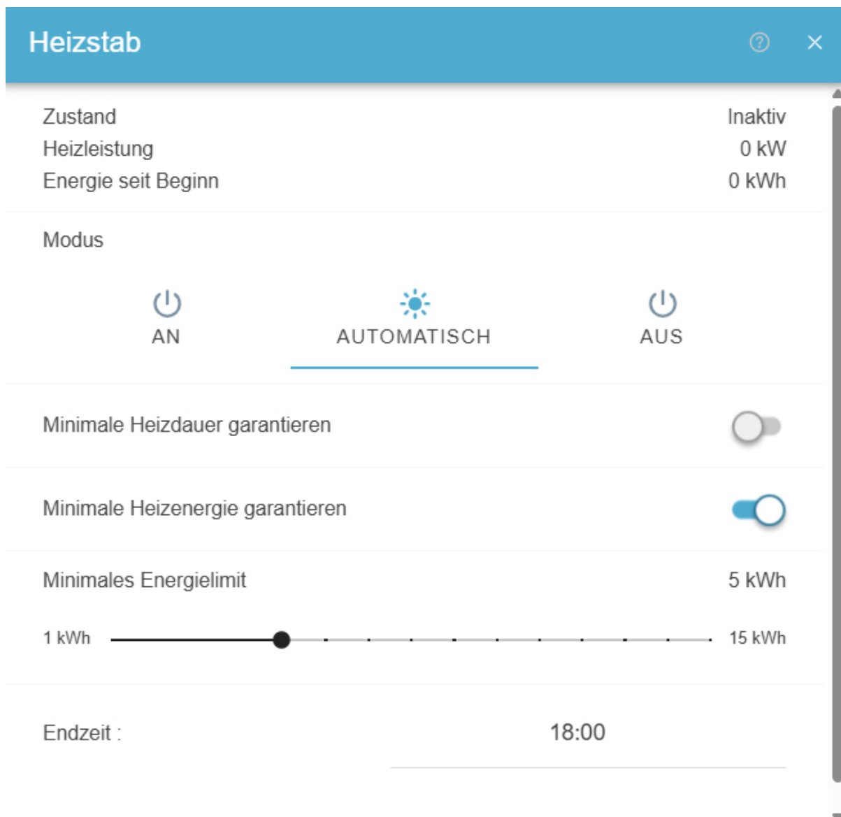
Image 13. Heating element — "Automatic" operating mode with meter
