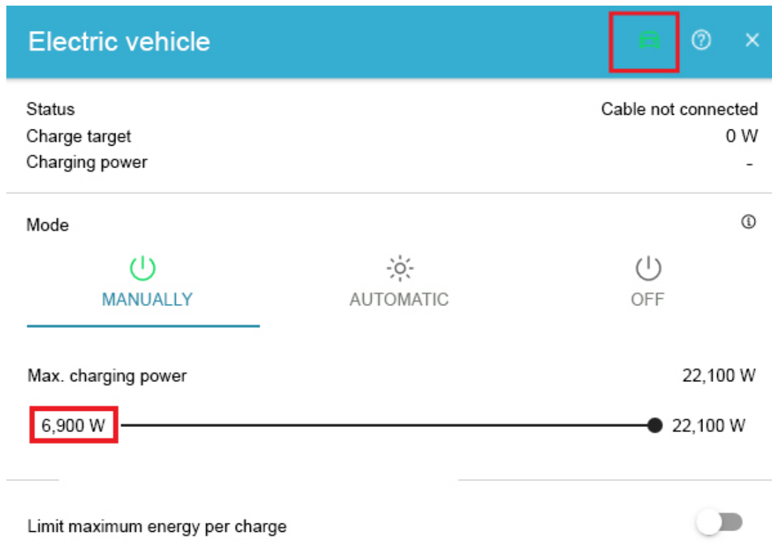
Figure 11. Vehicle management
