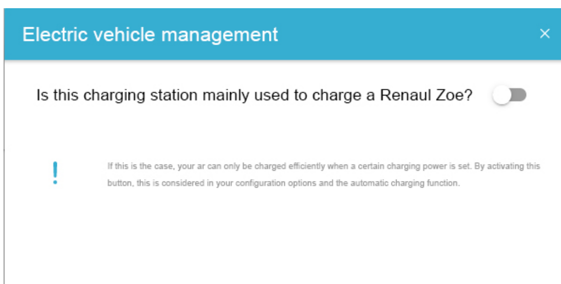
Figure 10. Vehicle management
