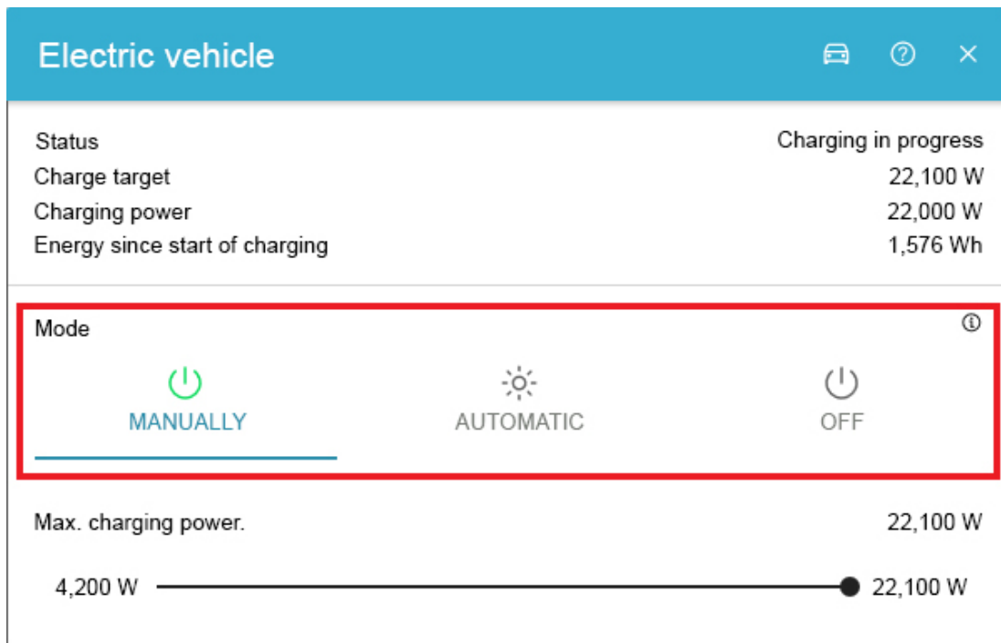
Figure 3. Detail widget
