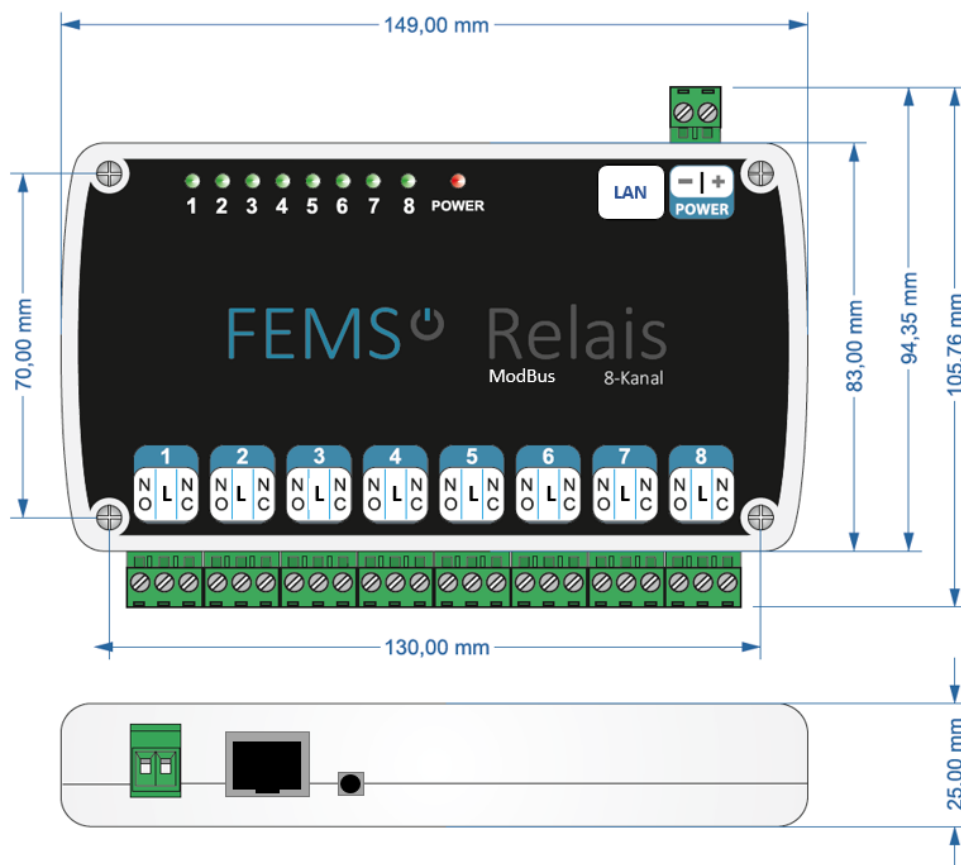
Figure 1. Abmessung FEMS Relaisboard 8-Kanal TCP
